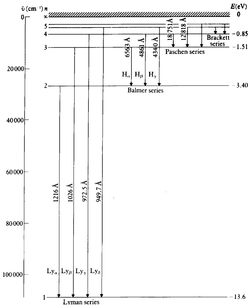
1.16 The spectrum of atomic hydrogen.
